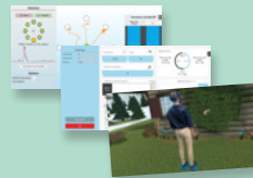
VR software
